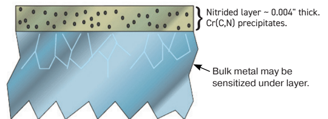
Conventional gas nitrided stainless steel
