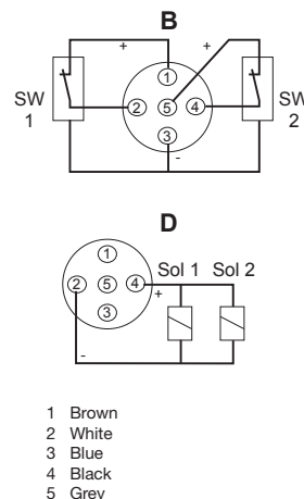
M12 Pinouts for P33
