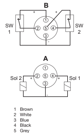
M12 Pinouts for P33
