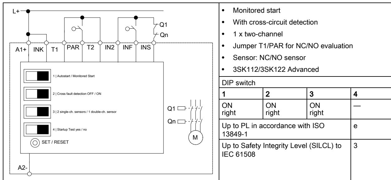
Typical circuit 14: 1NC/1NO sensor, with cross-circuit detection with monitored start
