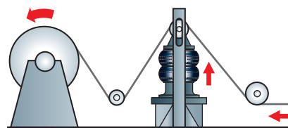
Web tensioning device
