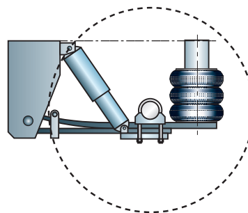
Wheel suspension
