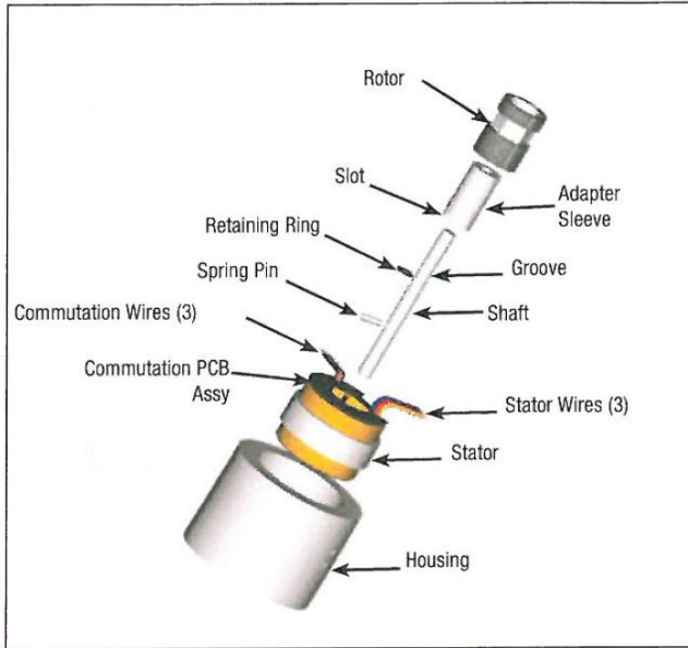
Spring Pin / Retaining Ring Method
