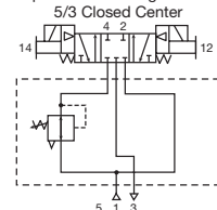
Independent Port Regulator with 5/3 Closed Center
