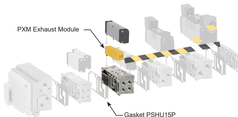
Gasket PSHU15P
