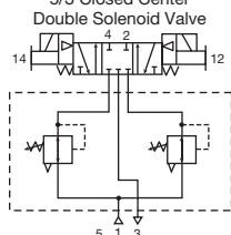
Independent Dual Port Regulator with 5/3 Closed Center
