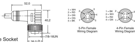
WKM Female Socket
