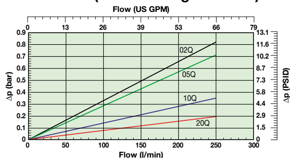
TPR200 (Element length code 6)
