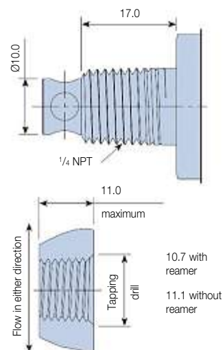
Installation details for 1/4 NPT
