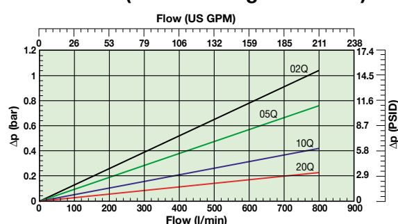
TPR650 (Element length code 11)
