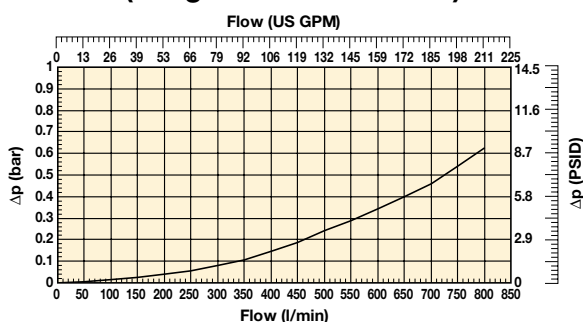
TPR III Empty Housing with G1½" ports (Length code 10 and 11)
