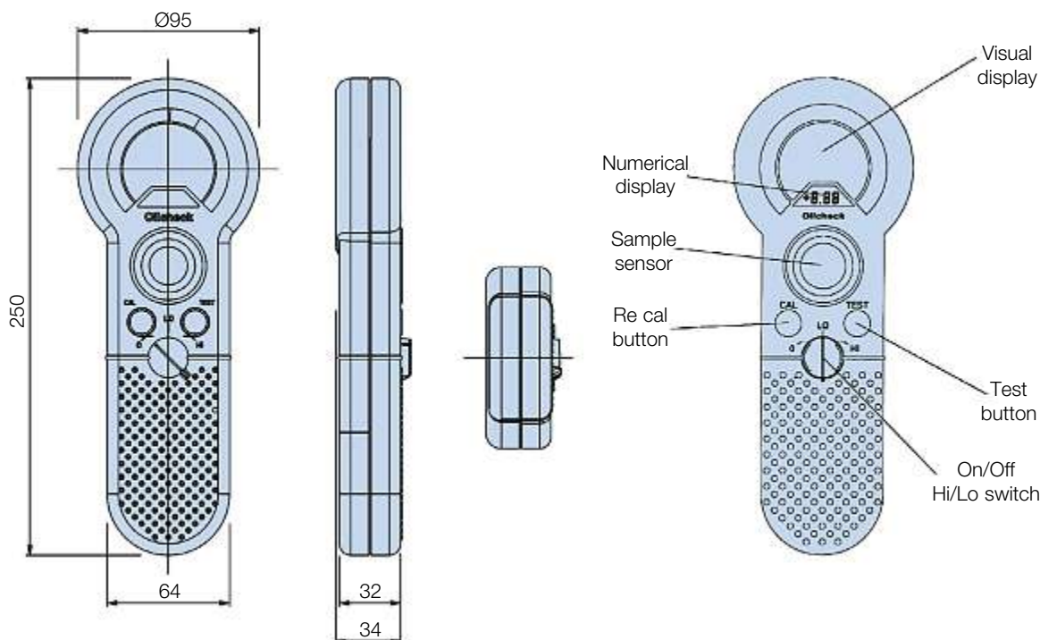
Function buttons
