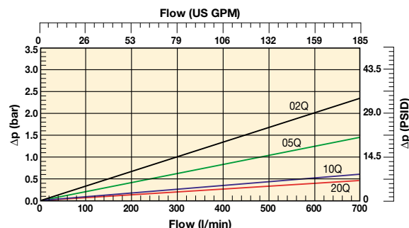
38P-2 High Collapse Elements
