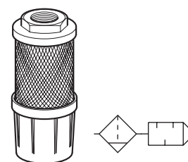
Central silencer
