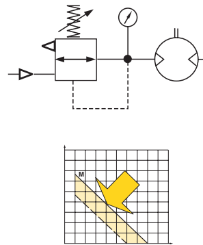
Pressure regulation at motor inlet.
