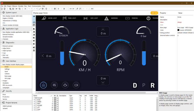
IQANdesign - display page HMI design
