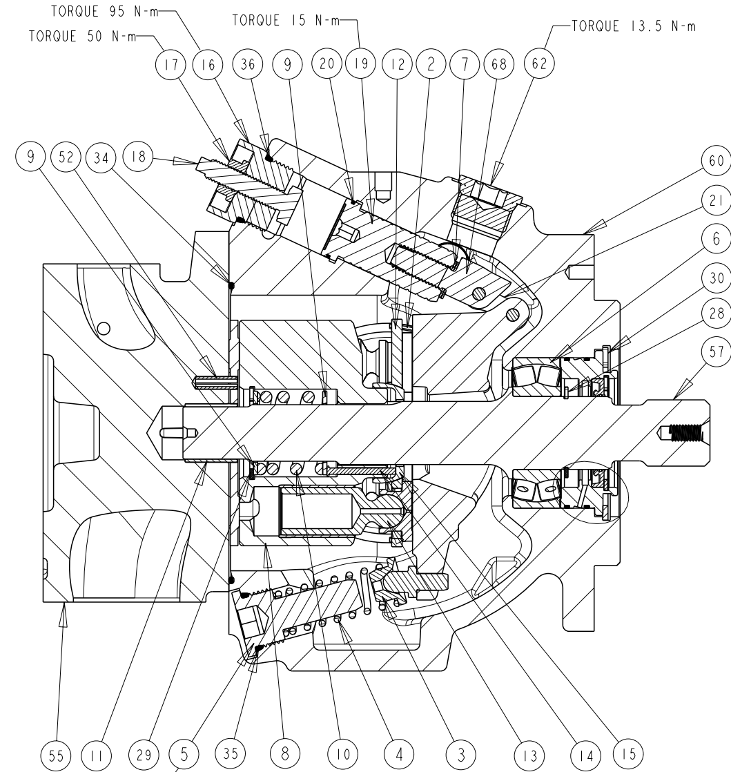
SECTION A-A SCALE 2:5
