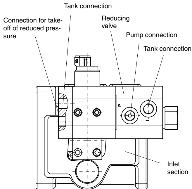
ESO/ESP on one spool section. Reducing valve fitted. Threaded connections for external take-off of reduced pressure, RA1 [48].
