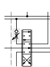
Adjustable restrictor and check valve in pressure gallery (MS or A16)
