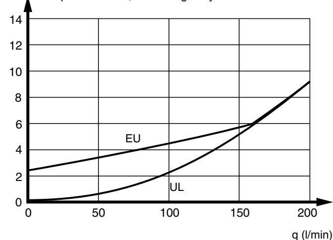
\Delta p (bar) Pressure drop pump-to-tank on emergency unloading. Spool actuated, free-flow gallery blocked.
