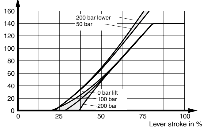
q(l/min) Flow rate in service port
