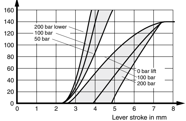
q(l/min) Flow rate in service port
