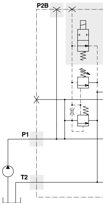
Inlet equipped with EU12/EU24 electric pump unloading. Energising the solenoid closes the unloading valve.
