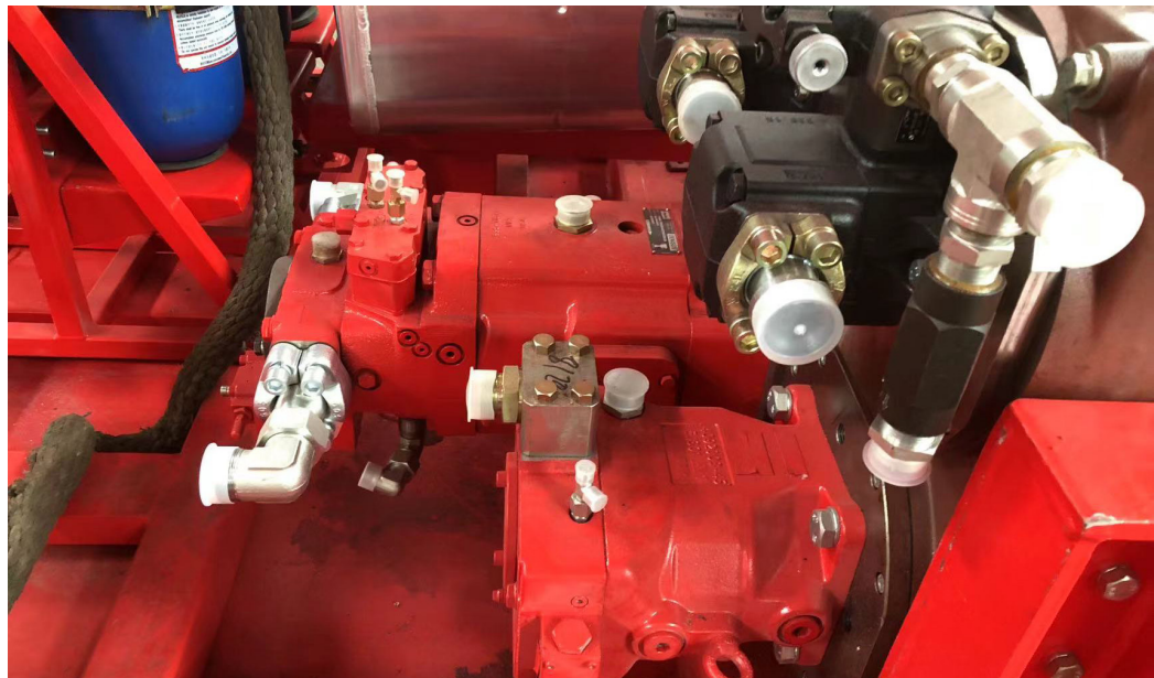
Parker's Gold Cup located in the Fracturing Truck's fan cooling system
