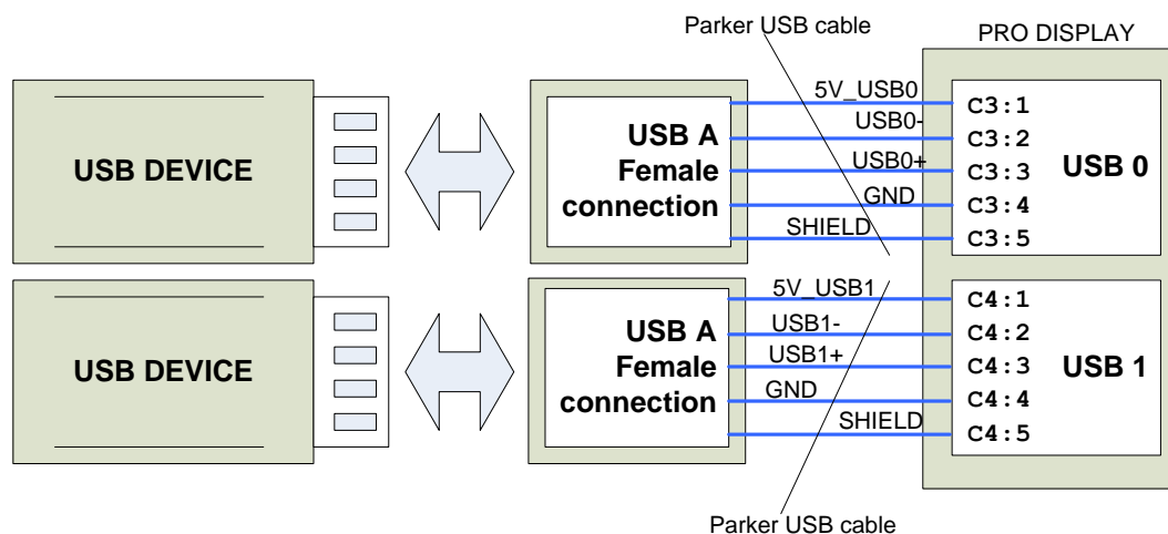
Figure 13: USB device/stick connection. USB 0 & USB 1 interfaces utilises M12 connector in Pro Display. M12 to USB cable adapter is available from Parker and the interface can be brought into the dashboard or other suitable place in the vehicle cabin.
