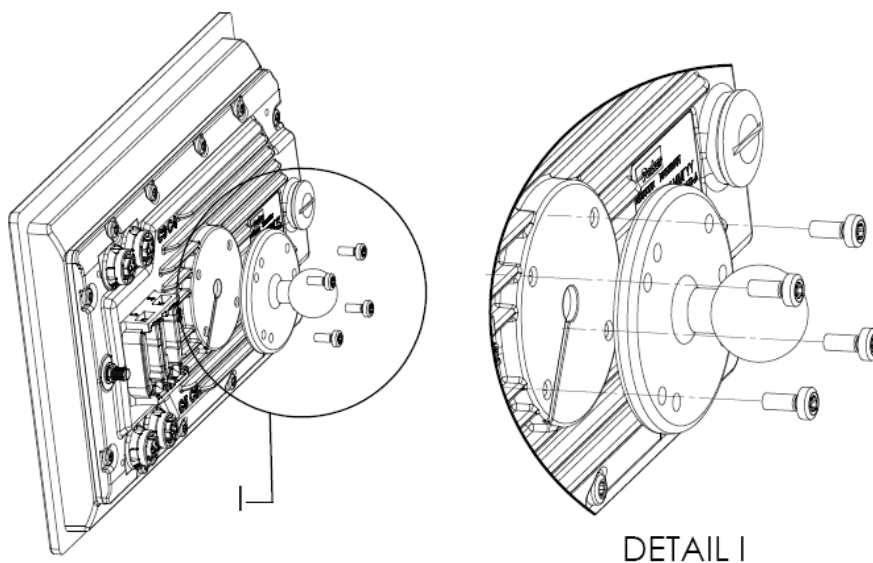
Figure 20: Pro Display 10 swivel mount method using RAM ball. First RAM ball is installed into rear side of the Pro Display and the second RAM ball into assembly surface of the vehicle.
