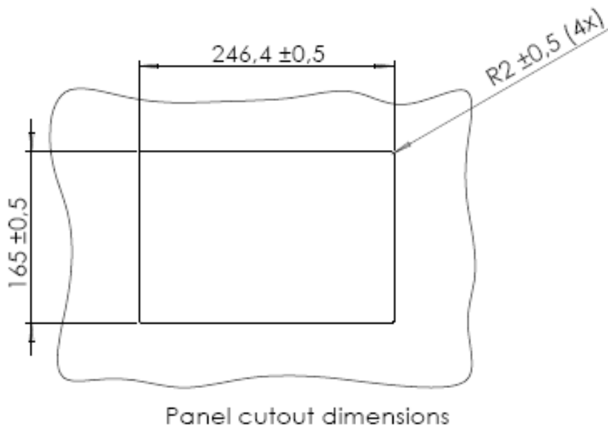
Figure 19: Cutout dimensioning for panel mounting.
