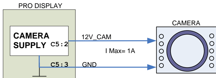
Figure 10: Camera supply output. When there is second camera in the end application, the branching of the supply wires shall be implemented in a wire harness – see more about this in figure 7, chapter 4.4.
