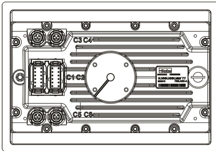
Figure 22: Pro Display back cover with connectors
