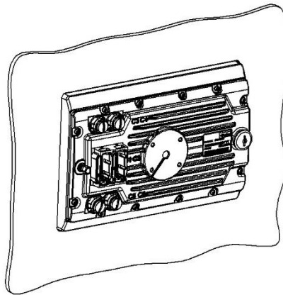
Figure 18: Pro Display 10 panel mount method. This assembly is intended for assemblies where the installer can operate behind the assembly surface – for example cabinet doors.
