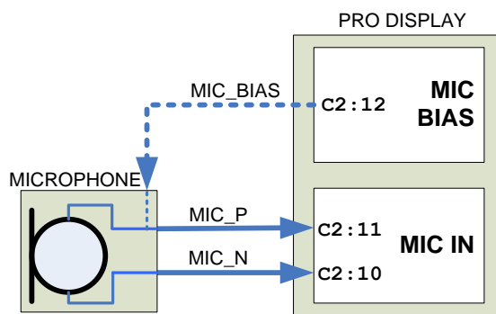
Figure 6: Pro Display microphone input
