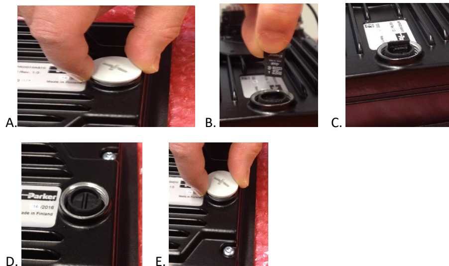
Figure 27 (subfigures A to E): Micro SD card installation into connection C1 on the rear side of the Pro Display
