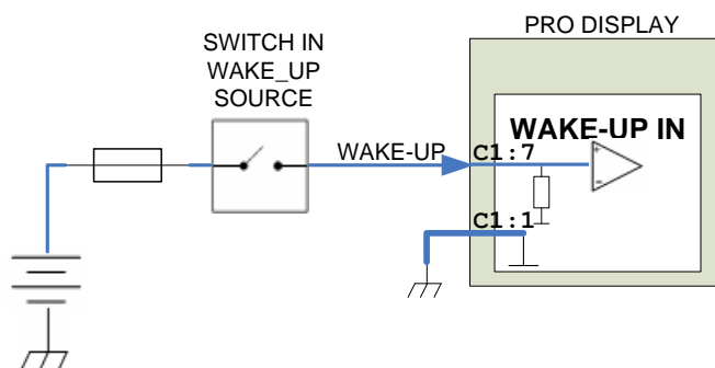
Figure 9: Wake-up input connection principle
