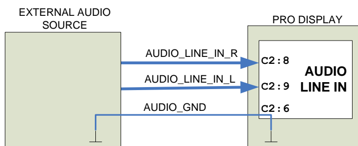
Figure 4: Line input
