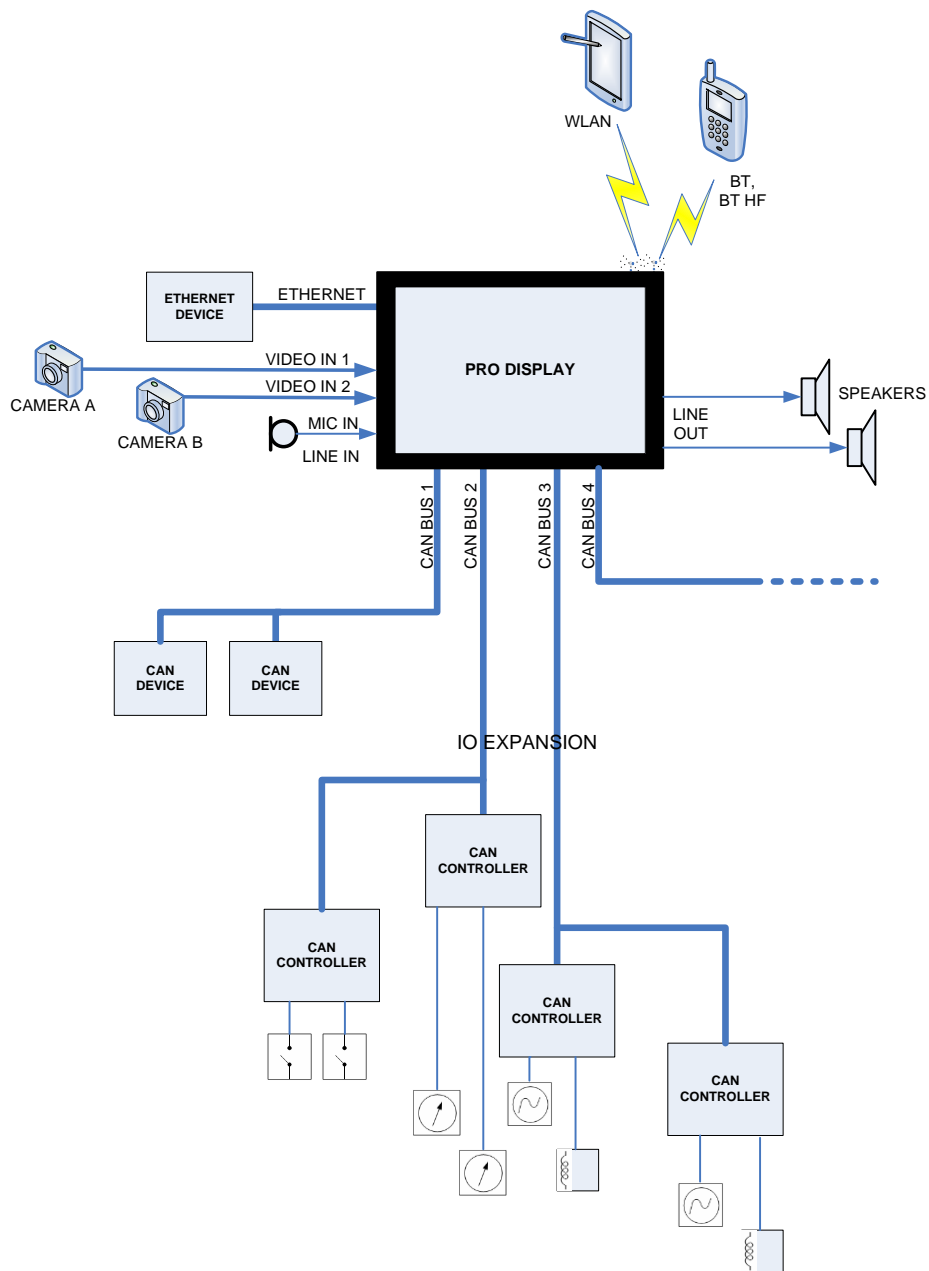
Figure 3: Pro Display system overview. This figure shows just one possible application.
