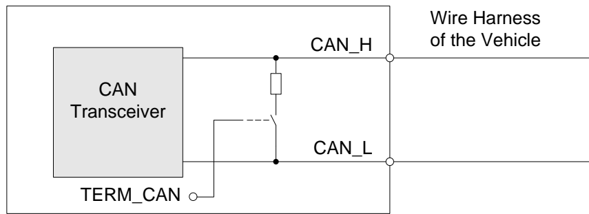
Figure 12: Software controllable CAN termination feature in Pro Display
