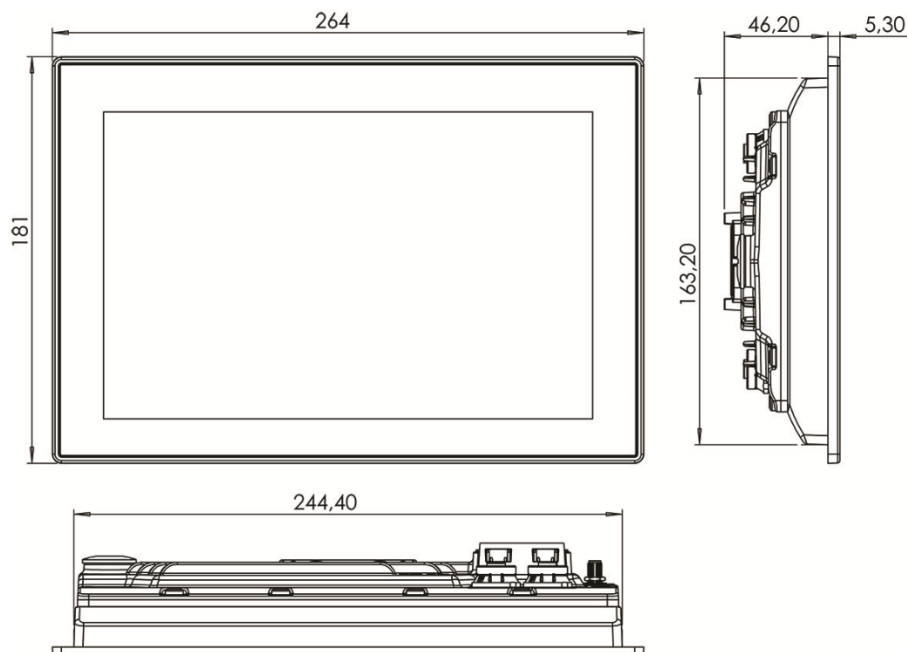
Figure 17: Pro Display 10 dimensions
