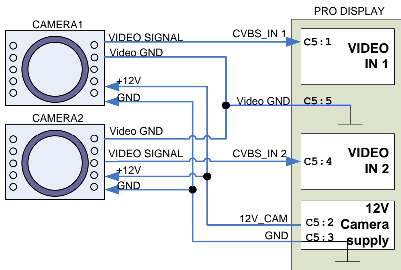
Figure 7: Video Camera connection principle for 2 cameras
