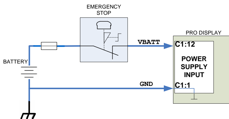
Figure 29: Emergency stop connection principle
