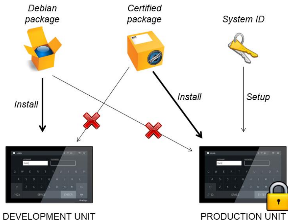
Figure 14: Installing packages – overview
