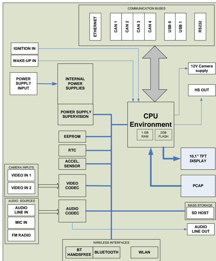
Figure 2: Pro Display block diagram
