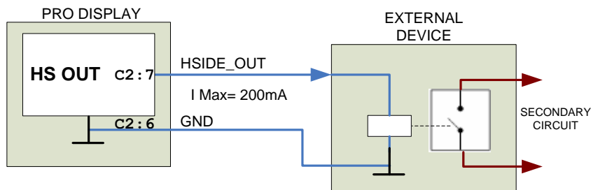
Figure 11: High-side output connection principle. This shows just one use case for this output; an external device can also be an indicator etc.
