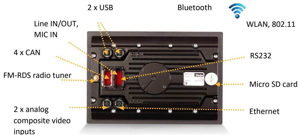
Figure 23: Pro Display interfaces
