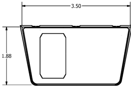
Updated Bracket (PN 380668X)
