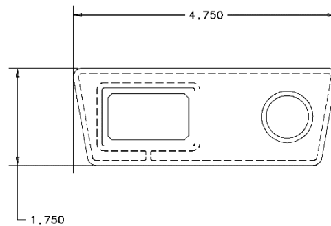
Legacy Bracket (PN 379336)
