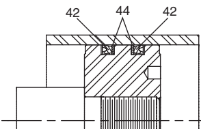
Lipseal Piston (All Series)
