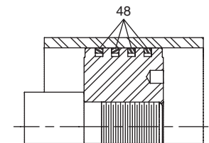
Ring Type Piston (All Series except 2A)
