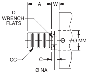
Thread Style 8
