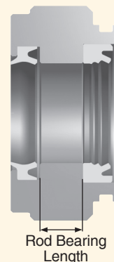
Pilot Gland
