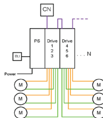
TPD-M solution: one drive for three axis in a rack solution. Only one Power Supply
