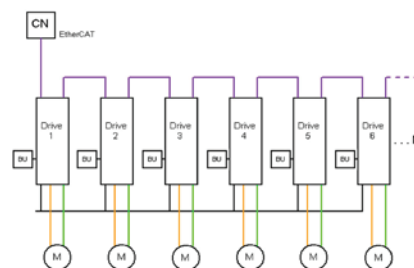
Traditional solution: one drive for each axis
