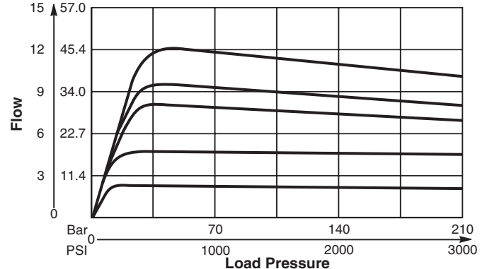
Pressure Compensation of Regulated Flow GPM LPM Hydraulic Oil 150 SSU @ 100°F (32 cSt)
