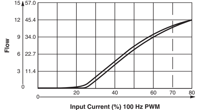
GPM LPM Hydraulic Oil 150 SSU @ 100°F (32 cSt)
