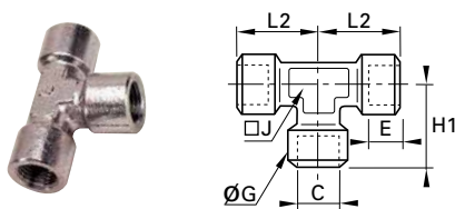
1845 Equal Tee Female BSPP
