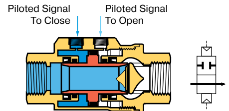
Piloted State (Valve Closed)
