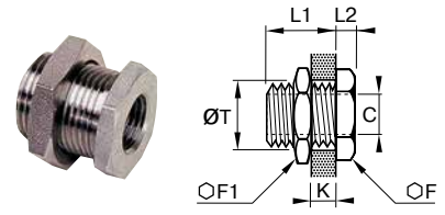
1871 Bulkhead Adapter NPT
