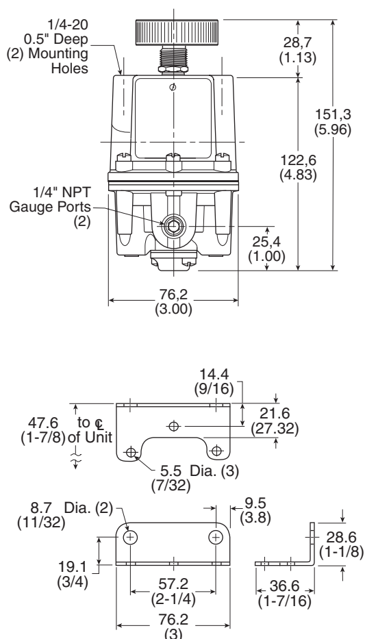
Mounting bracket
