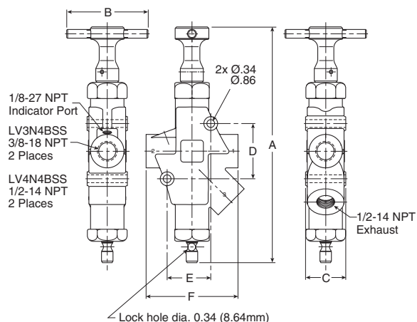
Stainless Steel LV Series, 1/2" Exhaust Port Dimensions
