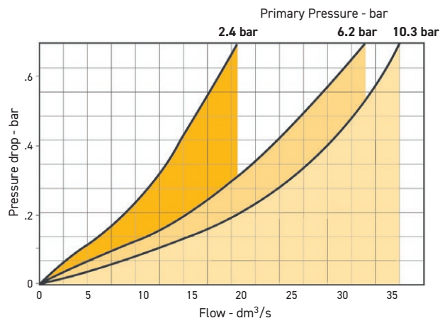
Flow Characteristics - 1/2 Inch Ports PF11-04DJSS
