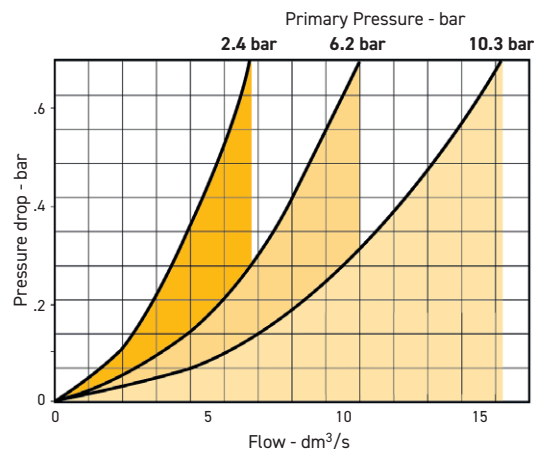
Flow Characteristics - 1/4 Inch Ports PF501-02DHSS
