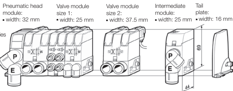
Typical T series islands combining different valve flows and functions
