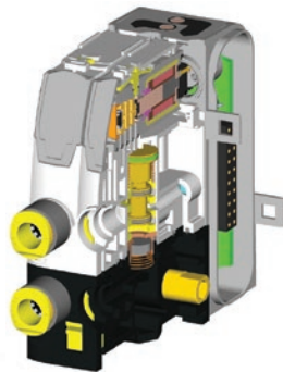
Dual 4/2 valve
