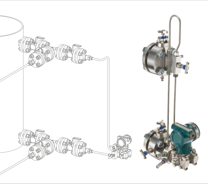
This assembly combines wet and dry leg installations. The close coupled assembly mounted at the bottom of the tank consists of an instrument manifold and a piping isolation monoflange in a single-piece machined unit and the differential pressure transmitter directly mounted onto it. The assembly is connected to the high pressure leg (or wet leg). The low pressure (or dry leg) is connected to the monoflange and manifold assembly at the top of the tank. Please consult your local Parker support.
