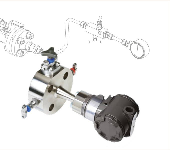
This assembly utilises a Coplanar™ bolted interface between the flanged outlet and the transmitter. Please consult your local Parker support.
