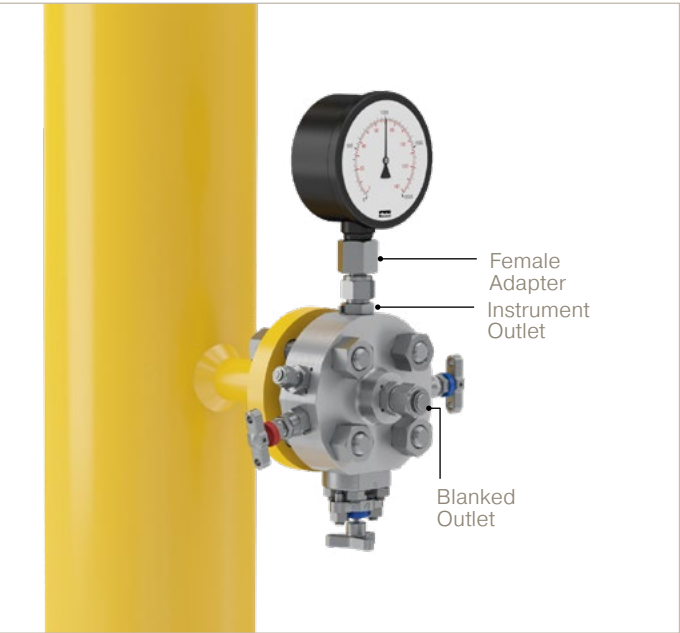
Monoflange with a dual outlet option mounted directly to a vertical pipe.
