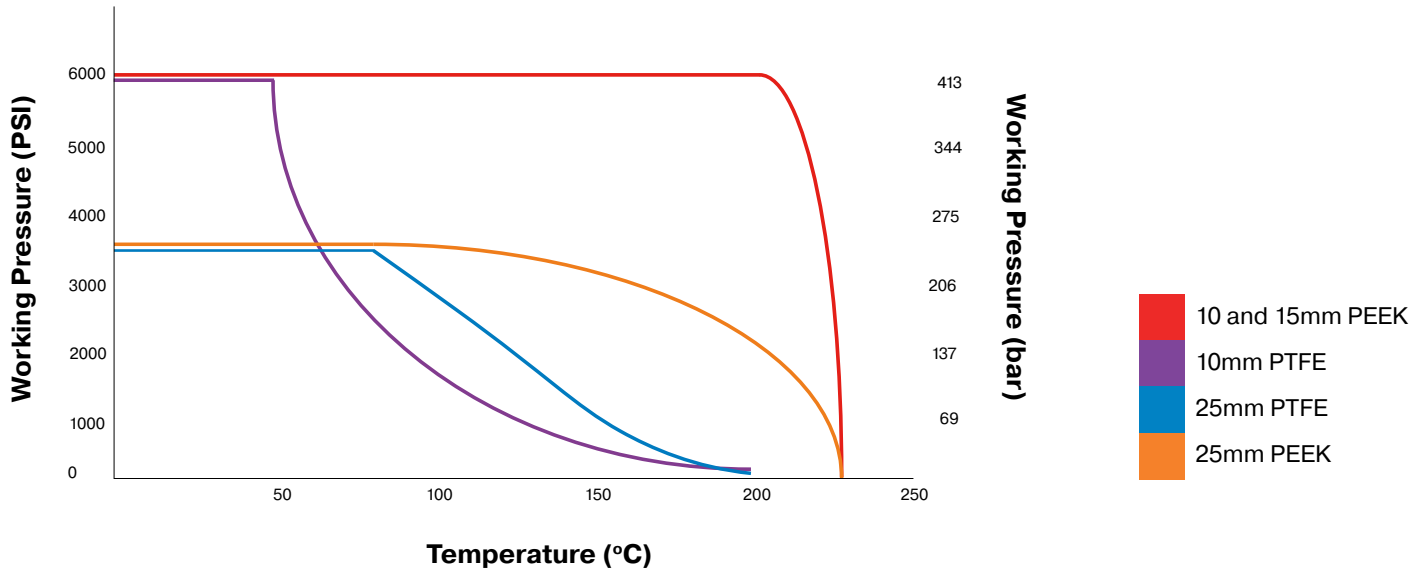
Pressure-Temperature Ratings for Seats
