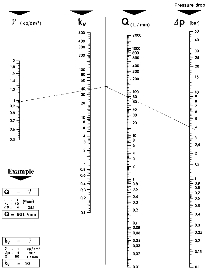
Nomogram for liquid flow calculation
