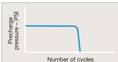
Fig. 15 When an accumulator bladder ruptures, precharge pressure immediately falls to zero
