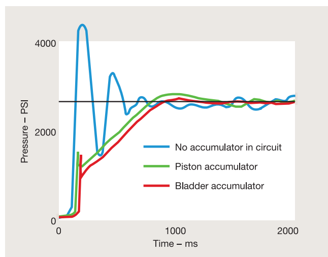
Fig. 5 Shock wave test results – Example 2
