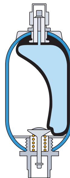
Fig. 6 A horizontally mounted bladder accumulator can trap fluid away from the hydraulic valve
