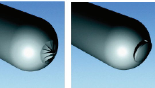
Fig. 11 (Left) Starburst rupture caused by loss of bladder elasticity
