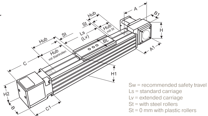
LBB with toothed belt without steel strip cover
