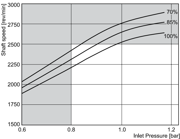
P3145 Inlet characteristics
