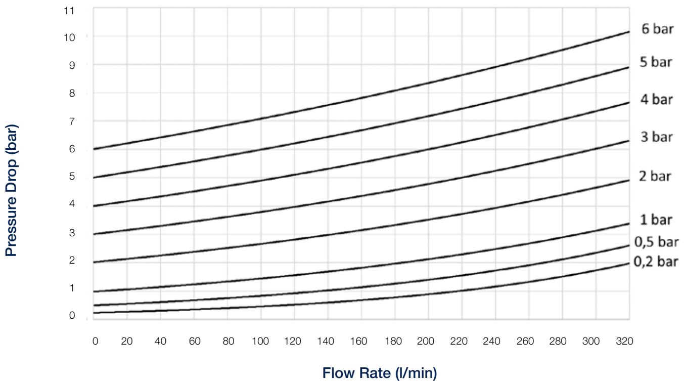
Pressure Drop Tube O.D. 35+42L/38S; size 24; female BSPP 11/2; RVP 55; DN 29
