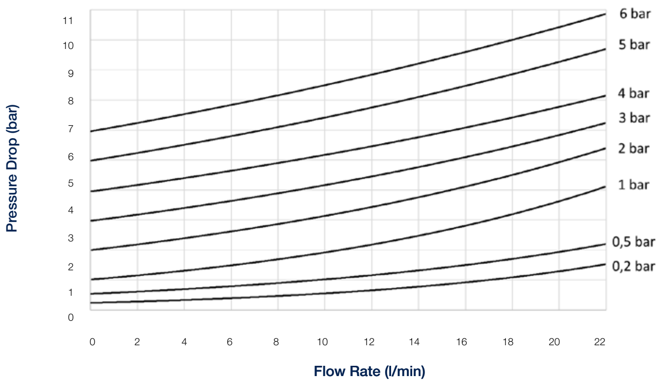
Pressure Drop Tube O.D. 10L/12S; size 6; female BSPP 3/8; RVP 20; DN 7.5
