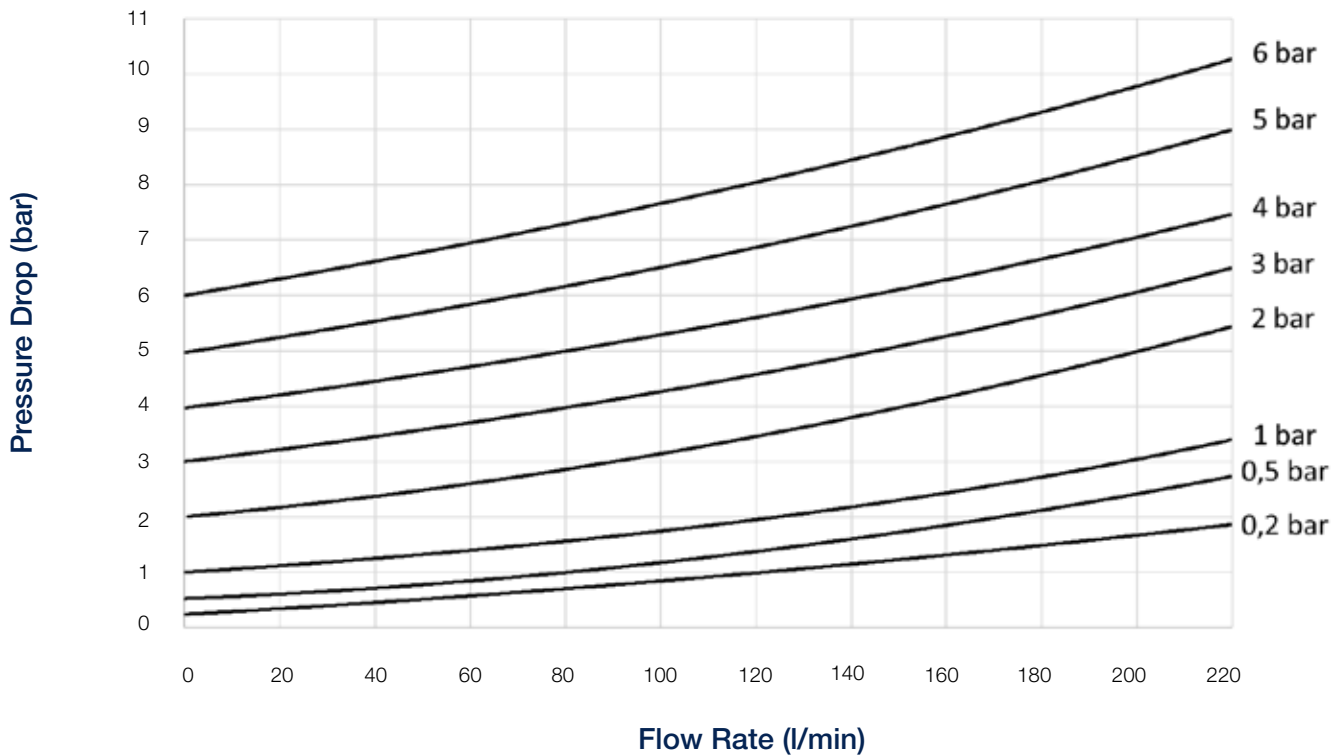
Pressure Drop Tube O.D. 28L/30S; size 20; female BSPP 11/4; RVP 47; DN 24
