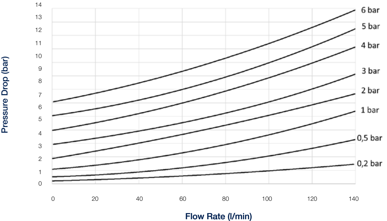
Pressure Drop Tube O.D. 22L/25S; size 16; female BSPP 1; RVP 40; DN 19
