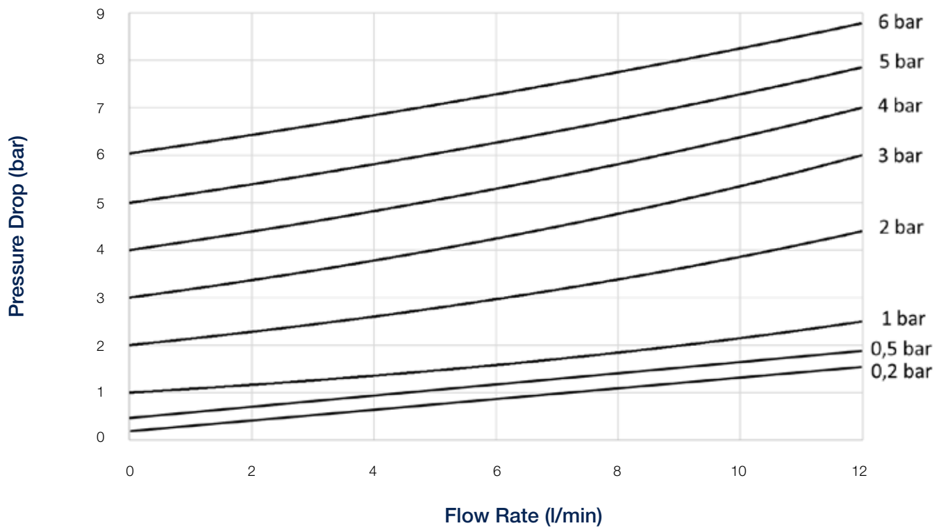
Pressure Drop Tube O.D. 08L/10S; size 5; RVP 16; DN 5.5
