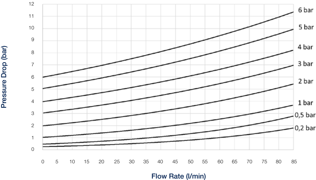
Pressure Drop Tube O.D. 18L/20S; size 12; female BSPP 3/4; RVP 35; DN 15.0
