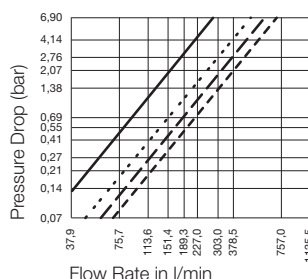
Flow Capacity with Hydraulic Oil 88 SSU with Viscosity of 18cSt
