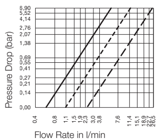
Flow Capacity with Water
