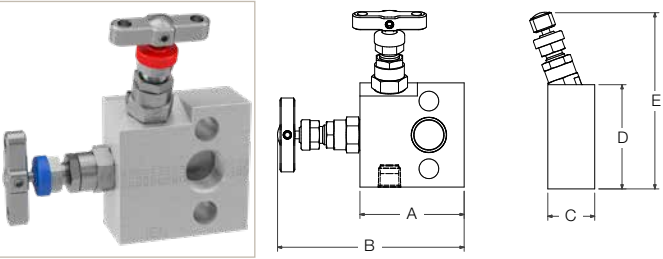
HD*2MFD variant available with vent/bleed/drain connection on same face as process inlet.
