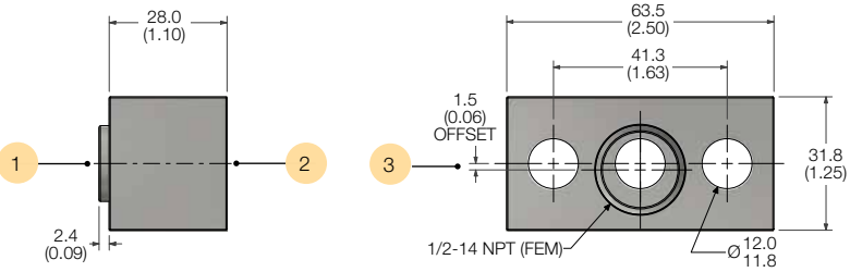
Example shown with traditional 1/2" NPT Fem. connection.
