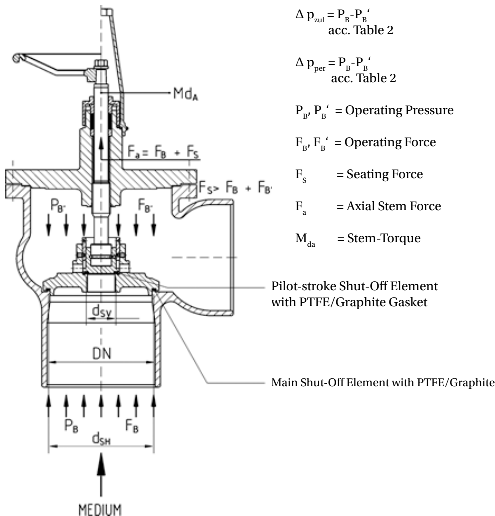
Figure 1 Sketch of a shut-off valve (Example: T6F.HUB)
