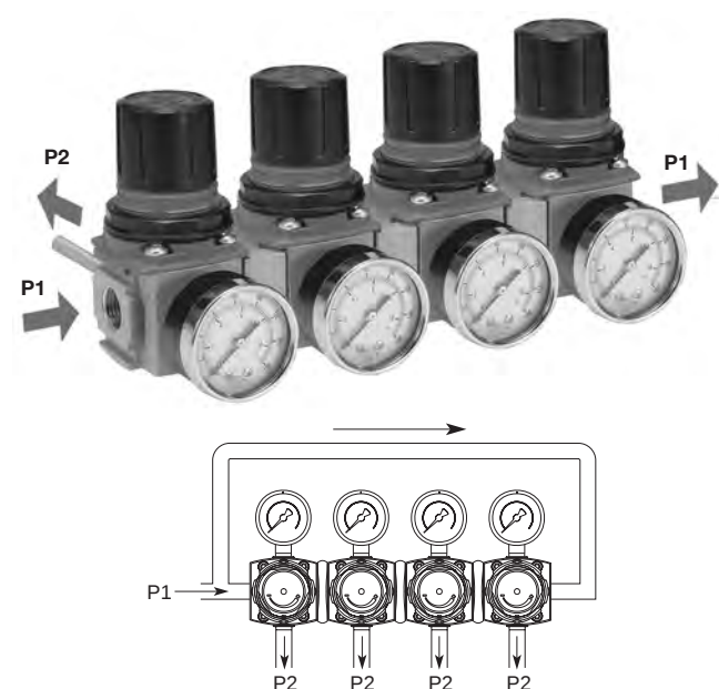
Self relieving regulator with gauge
