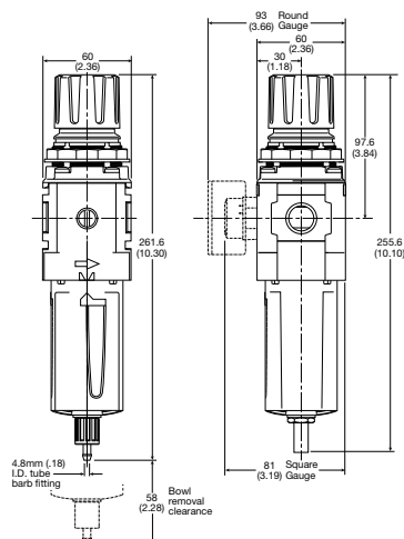
Manual Drain
