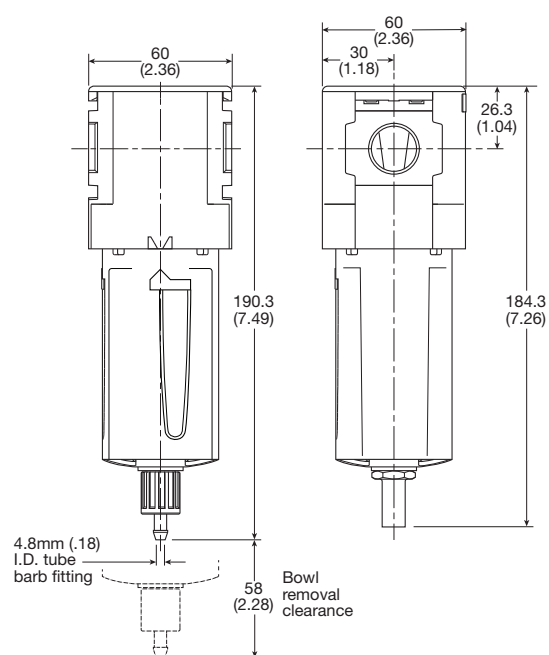
Manual Drain
