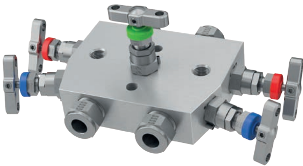
Example shown: 5-valve remote/line mount manifold featuring the Parker A-LOK® Superior Advantage Inverted integral tube fitting connections for the impulse line and NPT ported connections for the vent/drain.
