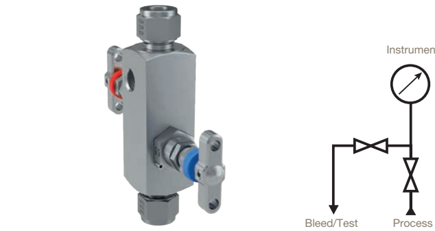
Example shown: 2-valve integral block and bleed manifold with integral A-LOK® connections.
