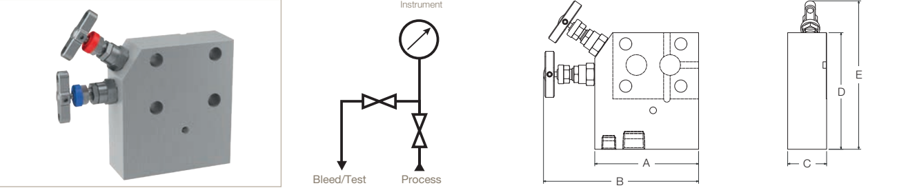
HD*2MCPEXT - Female threaded - NPT x Flanged
