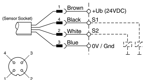
M12, 4-Pin, (2) PNP Outputs
