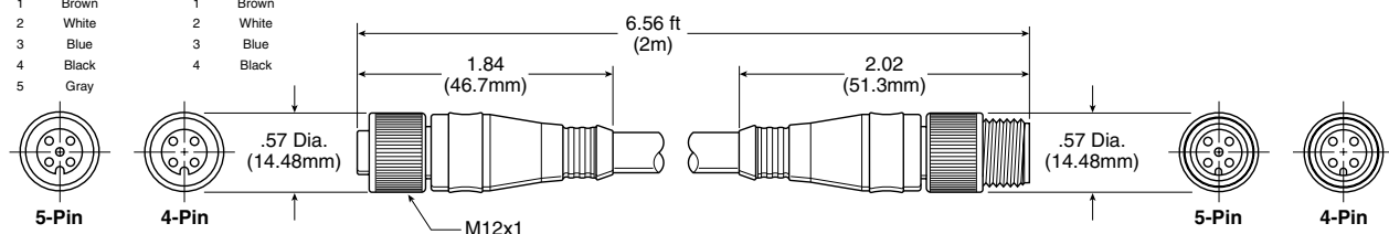
CB-M12-5P-M12-2M, Female to Male
