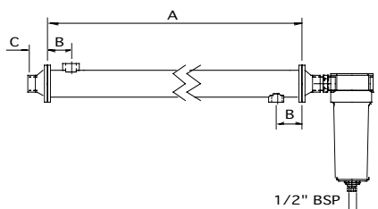
002-038 (WITH SEPARATOR STH)
