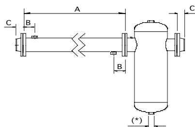
022-200 (WITH SEPARATOR SFH)
