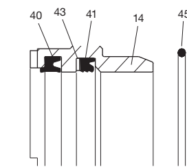
Gland Cartridge and Seals
