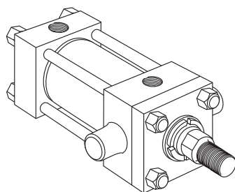
Style D Head Trunnion
