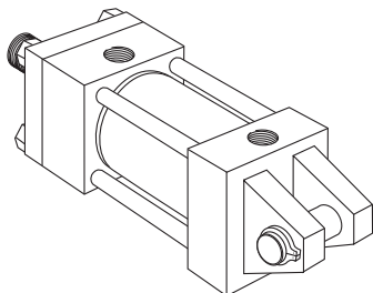
Style BB Cap Fixed Clevis ISO Style MP1
