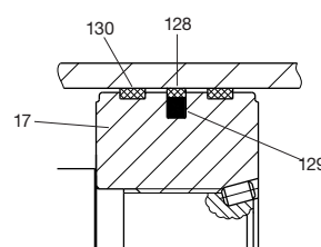
LoadMaster Piston
