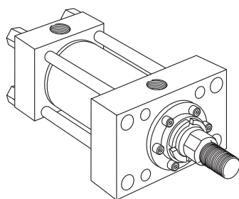
Style JJ Head Rectangular Flange
