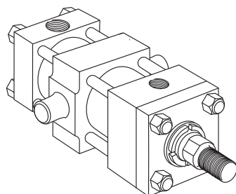
Style DD Intermediate Fixed Trunnion
