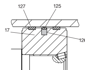
Standard Piston
