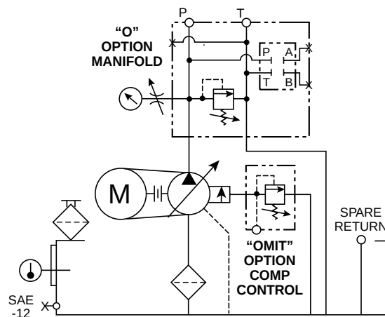
V-PAK BASIC UNIT
