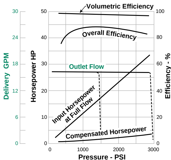
PVP33 @ 1800 RPM
