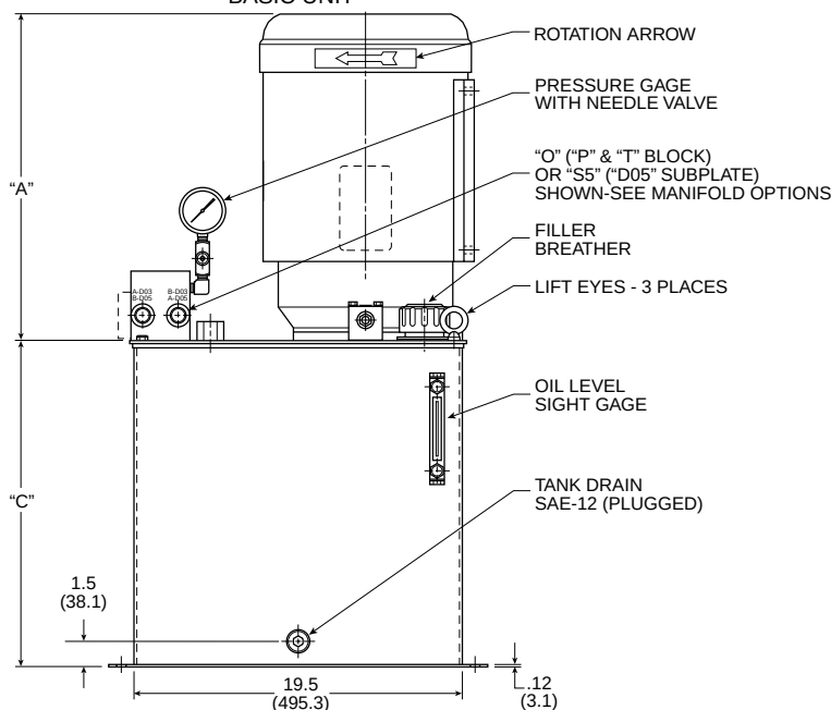
"O" & "S5" OPTION MANIFOLD (P & T BLOCK & D05 SINGLE STATION) BASIC UNIT
