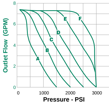
PVP16 @ 1800 RPM
