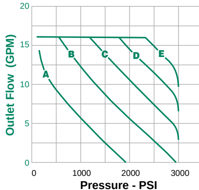
PVP33 @ 1800 RPM
