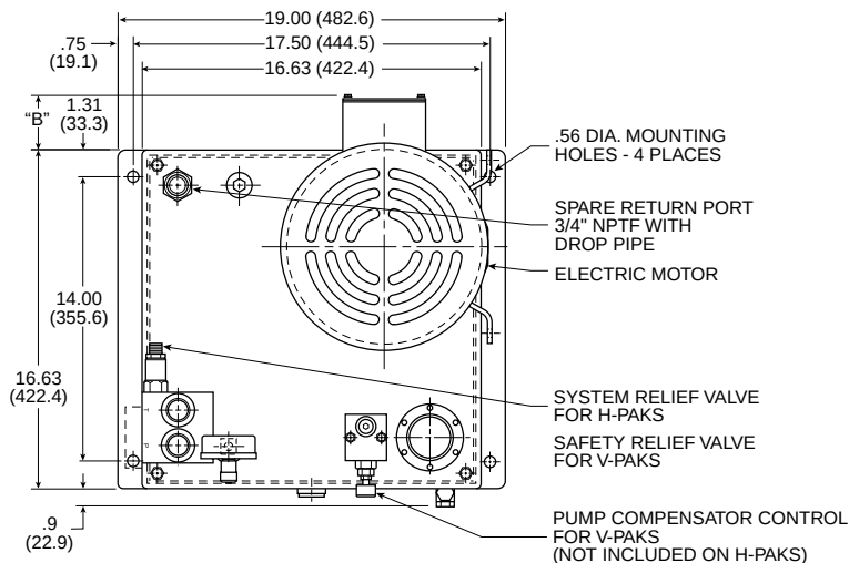
"O" & "S5" OPTION MANIFOLD (P & T BLOCK & D05 SINGLE STATION) BASIC UNIT
