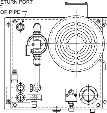
"O" & "S5" OPTION MANIFOLD (P & T BLOCK & D05 SINGLE STATION) SHOWN WITH OPTION "O" RETURN FILTER
