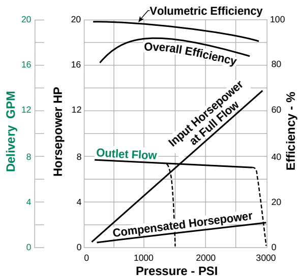
PVP16 @ 1800 RPM
