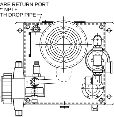
"M3*" OPTION MANIFOLD (MULTI-STATION D03 MANIFOLD) SHOWN WITH OPTION "O" RETURN FILTER
