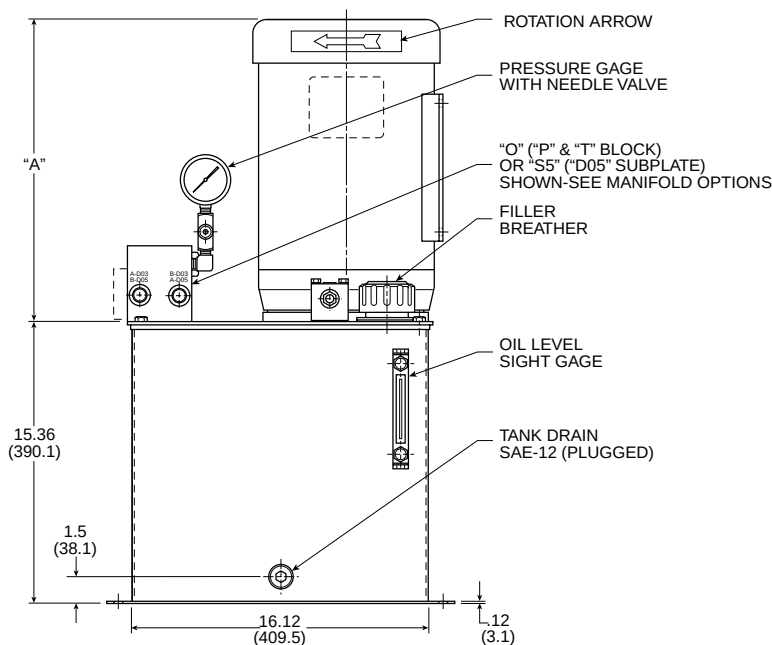
"O" & "S5" OPTION MANIFOLD (P & T BLOCK & D05 SINGLE STATION) BASIC UNIT
