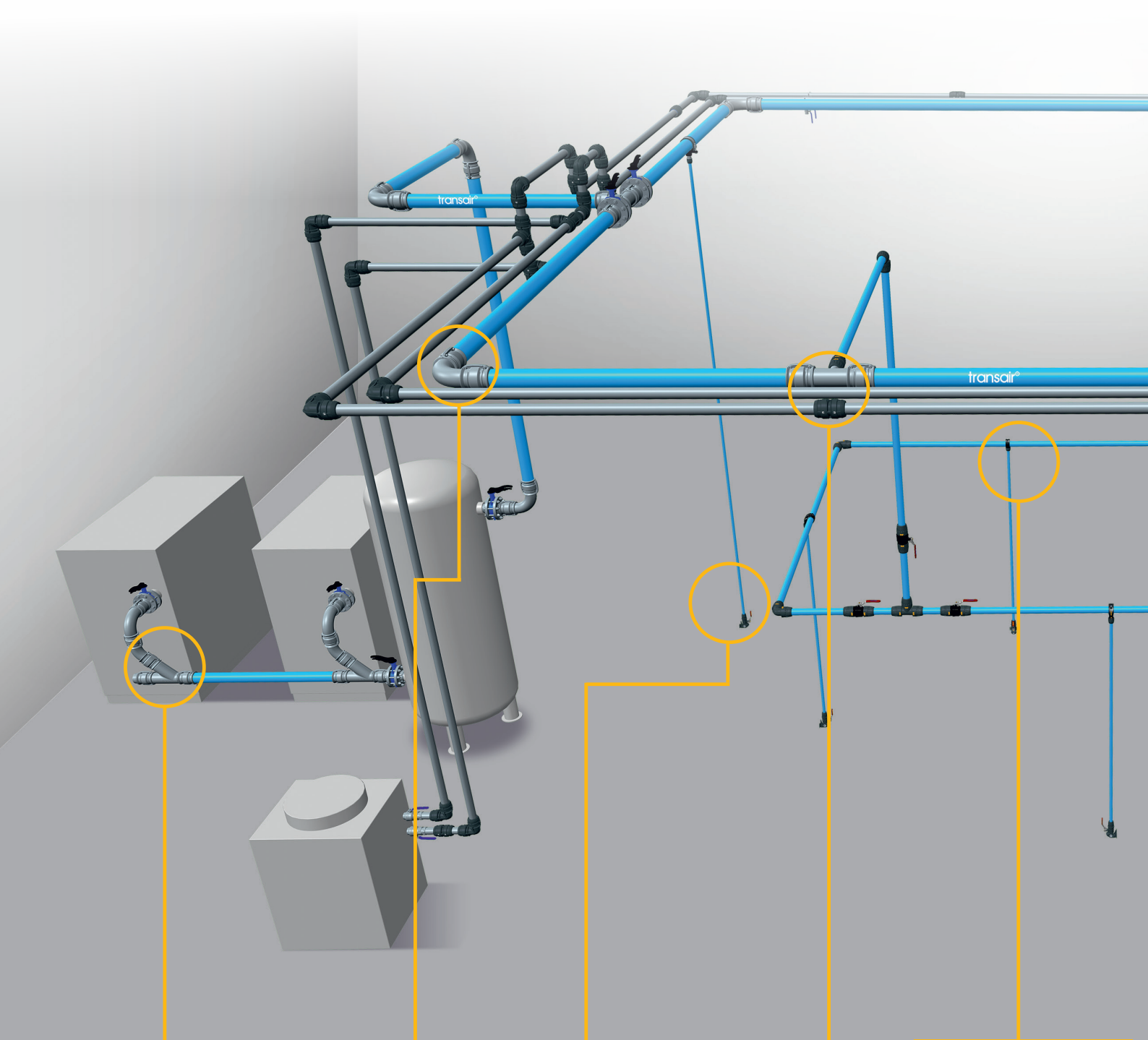
Technical Room
