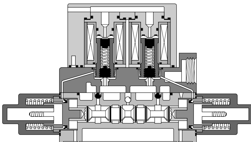
SS5010 Double Solenoid
