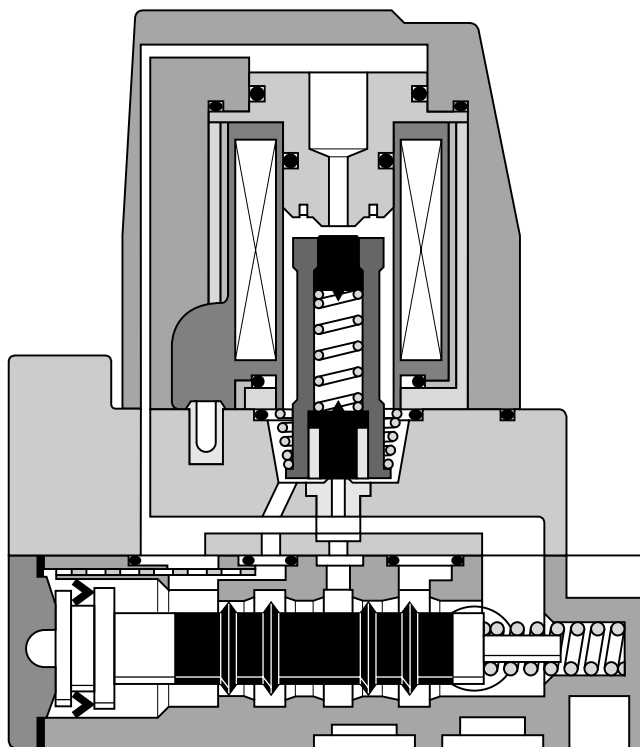
Single Solenoid Pilot GG-200B
