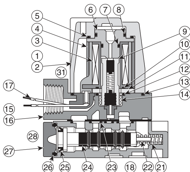
Figure 1: GG Valve Assembly
