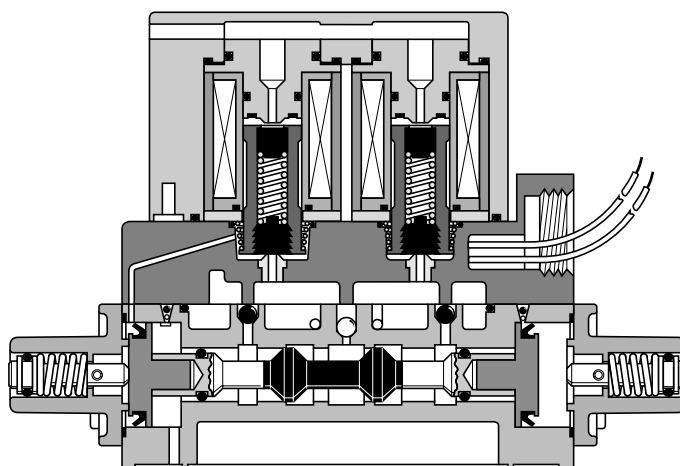
SS4010 Double Solenoid
