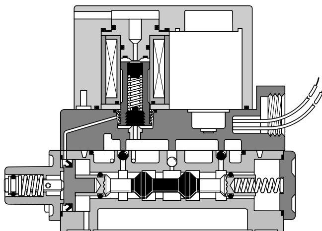
SS2010 Single Solenoid
