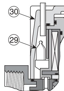
Figure 4: Indicator Lamp
