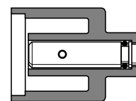
Figure 2: Flush Style Manual Override; Locking
