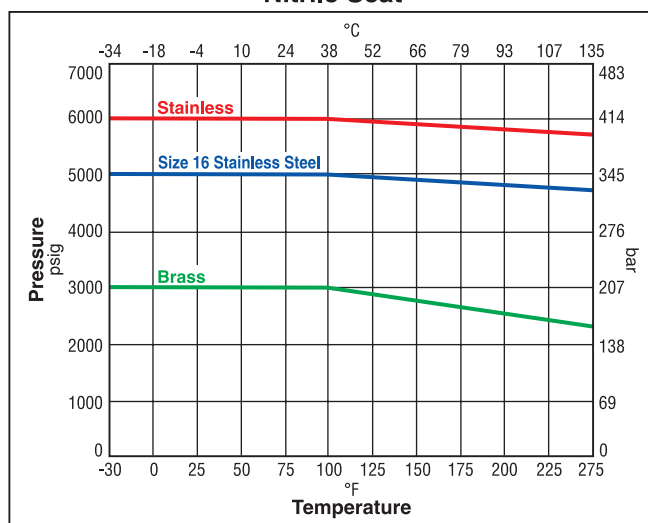
Nitrile Seat
