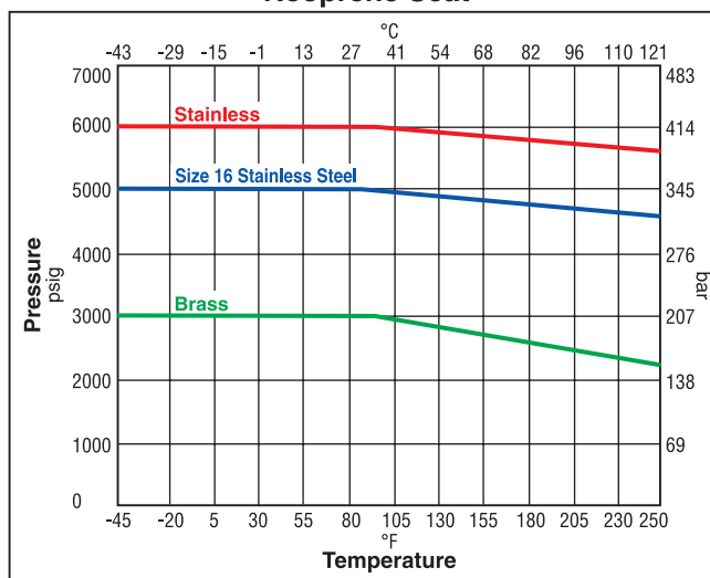
Neoprene Seat
