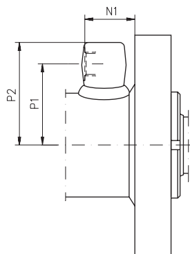
Alternative connection at piston-rod end, type C1. N.B. Dimensions as on page 4.
