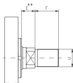
Piston-rod mounting provision type U. N.B. Dimensions as on page 4.
