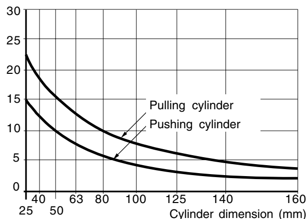
Friction losses (%)
