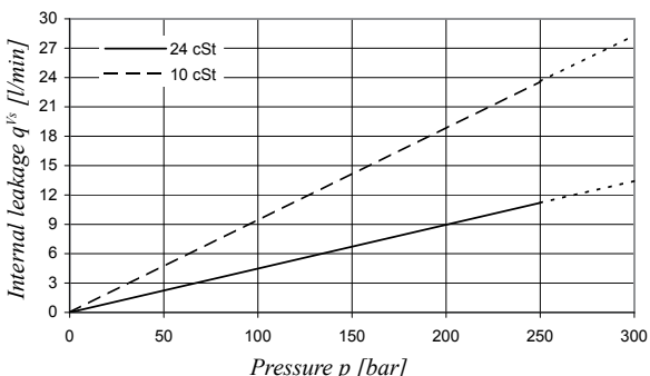
INTERNAL LEAKAGE (TYPICAL)
