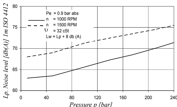
NOISE LEVEL (TYPICAL) - T7ES - 050
