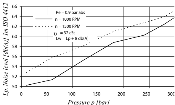
NOISE LEVEL (TYPICAL) - T7AS - B20
