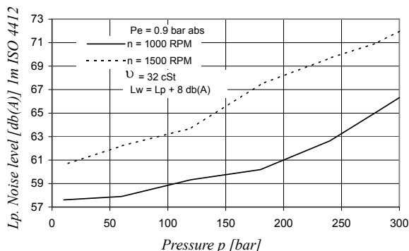
NOISE LEVEL (TYPICAL) - T7ASW B28
