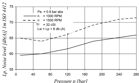
NOISE LEVEL (TYPICAL) - T7D - B31
