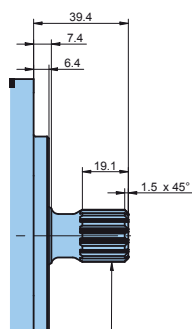
SHAFT CODE 3
