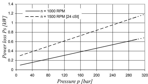
POWER LOSS HYDROMECHANICAL (TYPICAL)
