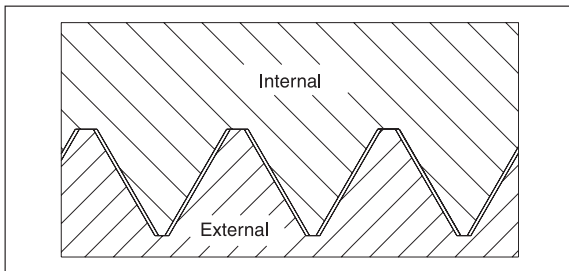
Fig. 3 – NPTF – Hand tight crest-root contact
