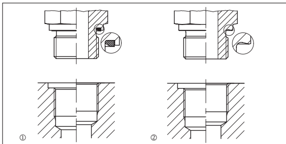
Fig. 10 – ① ED-seal; ② Form B
