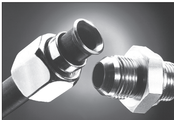
Fig. C1 – Assembled Triple-Lok® fitting cutaway and Triple-Lok® fitting components (fitting body with O-ring, sleeve and nut).
