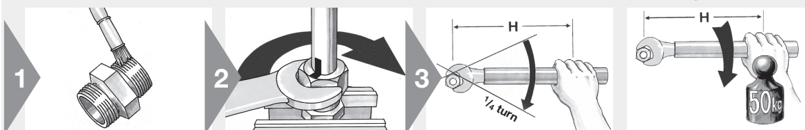
Spanner length
