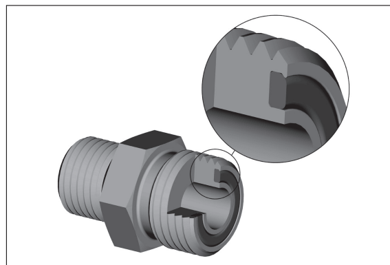
Fig 2 – Captive O-ring Groove (CORG) cutaway
