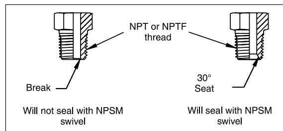
Fig. 12 – Illustration showing the required 30° seat on NPT/NPTF threads for NPSM swivel to seal
