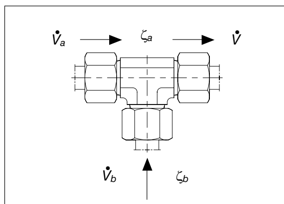
Pipe junction
