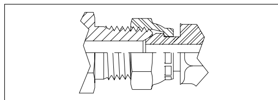
Fig. 11 – Illustration showing how NPSM swivel adapters seal on mating chamfer in male NPT thread
