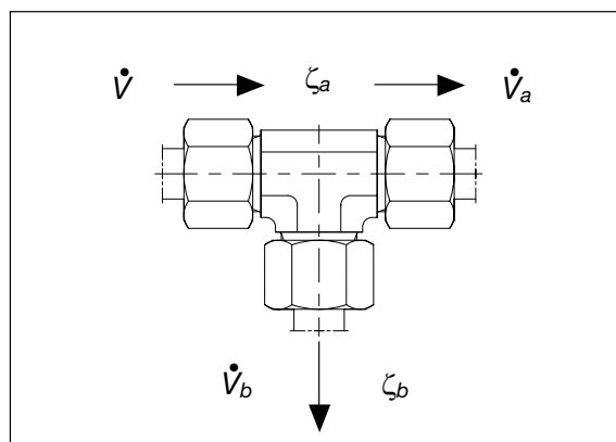
Pipe branching
