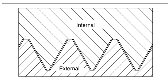
Fig. 3 – NPTF – Hand tight crest-root contact
