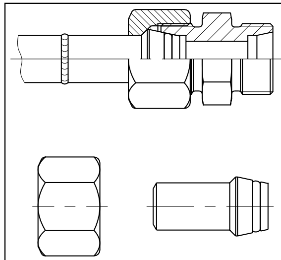
EO-Weld Nipples
