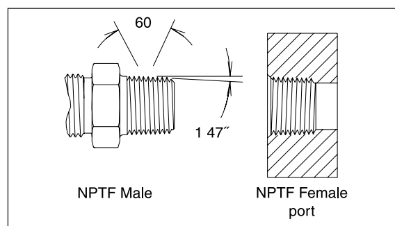
Fig. 1 – NPTF thread
