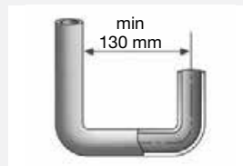
● Minimum clearance of U-shape bends
