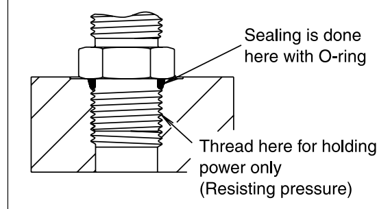
Fig. 6 – UNF port assembly
