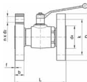
DN 32-DN50
