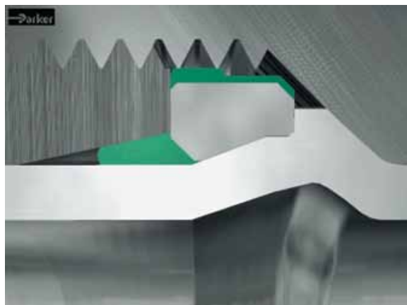
After tightening the nut
