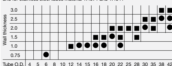
VH selection chart for EO Progressive Ring For steel tubes material ST 37.4 and for stainless steel tubes material 1.4571 and 1.4541
