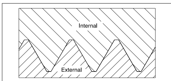
Fig. 4 – NPTF – Wrench tight crest-root and flank contact
