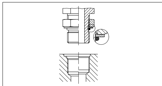
Fig. 7 – Adjustable UNF Port connection
