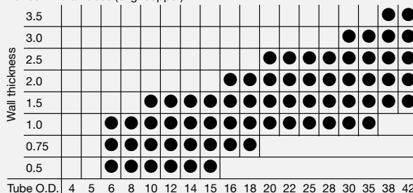
For soft metal tubes (e. g. copper)
