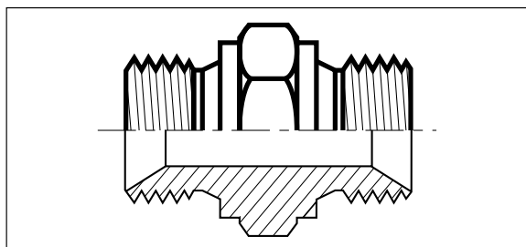
Fig. 9 – BSPP 60° cone adapter
