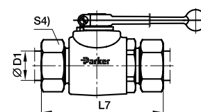
DN 32-40
