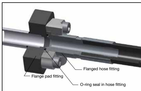
Fig. 1 – Flange pad fitting
