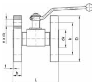
DN 10-DN25
