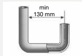
● Minimum clearance of U-shape bends
