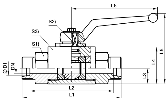
DN 4-25
