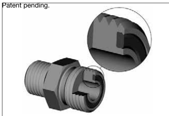
Fig 2 – Captive O-ring Groove (CORG) cutaway
